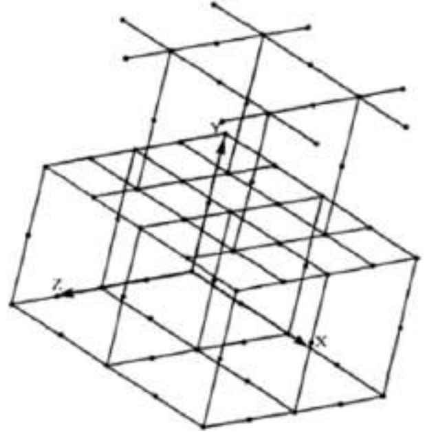
Fig. 10. A five-cell foam modeled with beam element [8].
