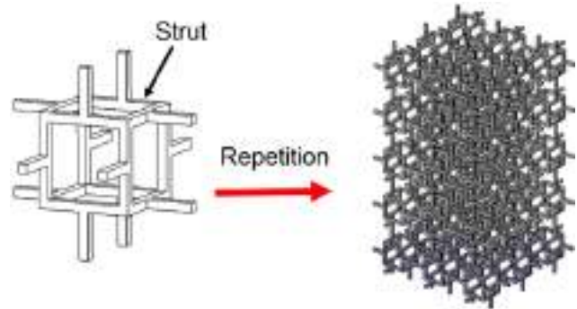
Fig. 1. Repetition of Gibson-Ashby cell and formation of open-cell foam.
