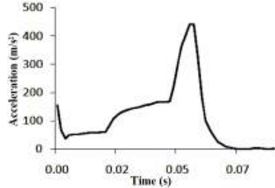
Fig. 19. Acceleration-time graph for the striker.
