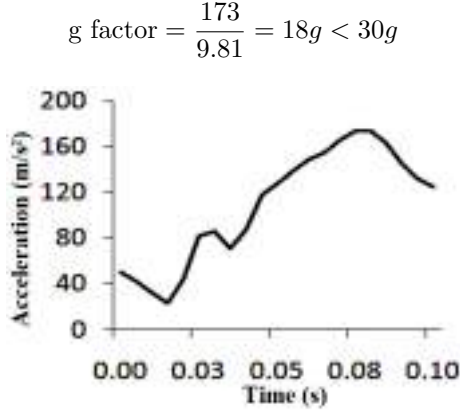
Fig. 24. Acceleration over time graph for the striker
