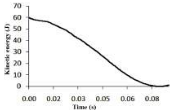
Fig. 22. Full absorption of kinetic energy of the striker by the foam.
