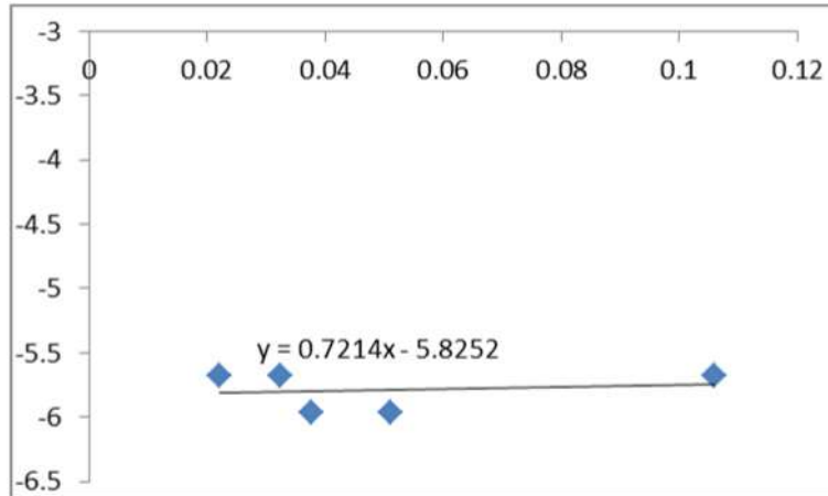
Fig 6: Plot of \ln\beta vs. \ln(1/\cos\theta) of sample milled for 10 h and heated at 1100 °C, 3 h
