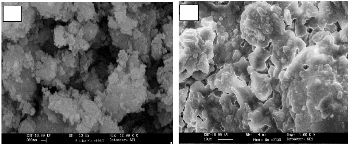
Fig. 3. SEM micrographs of the powder mixture milled for 10 h (A) and then heated at 1100 °C for 3 h (B)
