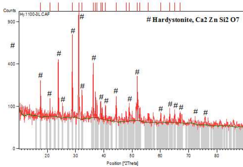
Fig. 5. XRD patterns of the materials milled for 10 h and then heated at 1100 °C for 3 h
