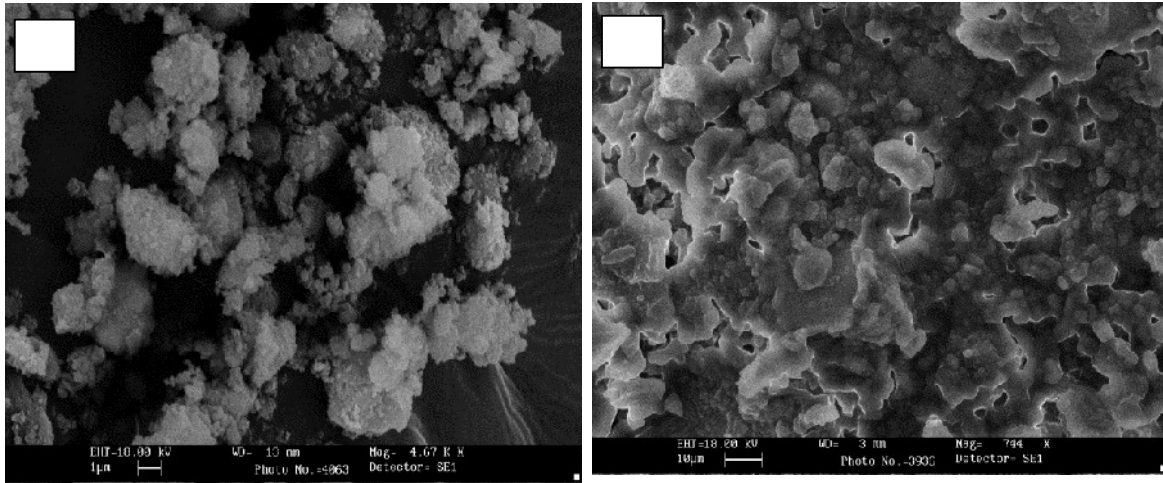
Fig. 2. SEM micrographs of the powder mixture milled for 5 h (A) and then heated at 1100 °C for 3 h (B)
