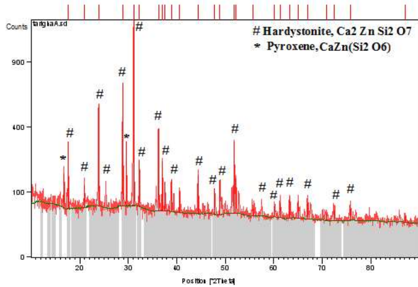
Fig. 4. XRD pattern of the materials mixture milled for 5 h and then heated at 1100 °C for 3 h
