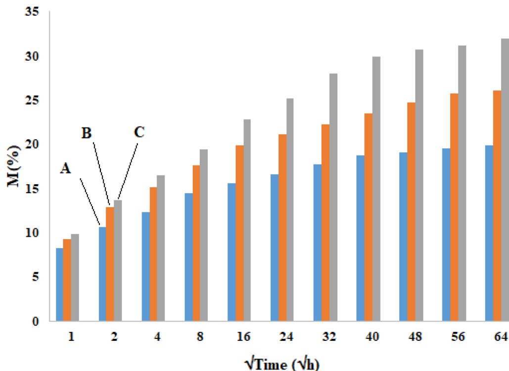
Fig. 3 Water adsorption potential of chitosan (A), chitosan-PEI (B), and chitosan-PEI-MTLTs polymeric systems (C).
