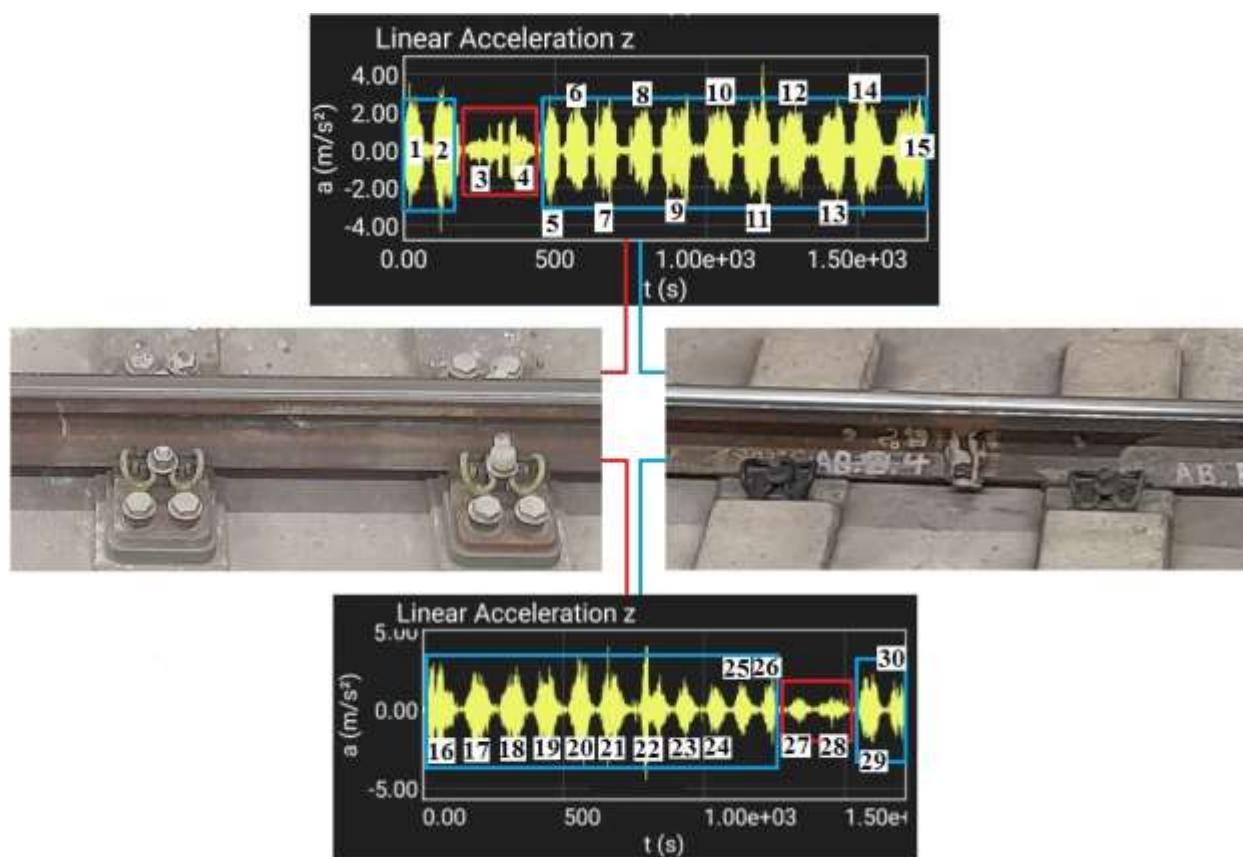
Fig. 8 Comparison of the vertical acceleration range with two different types of fastening systems.
