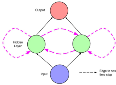
Fig. 5. Recurrent neural network model (Zeebaree et al., 2021).
