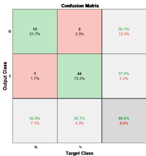
Fig. 10. Confusion matrix resulting from the proposed method after using the fusion technique.
