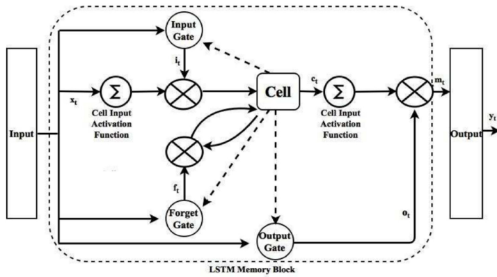
Fig. 6. LSTM network block diagram with three main gates: input gate, forget gate and output gate (Chauhan and Vig, 2015).
