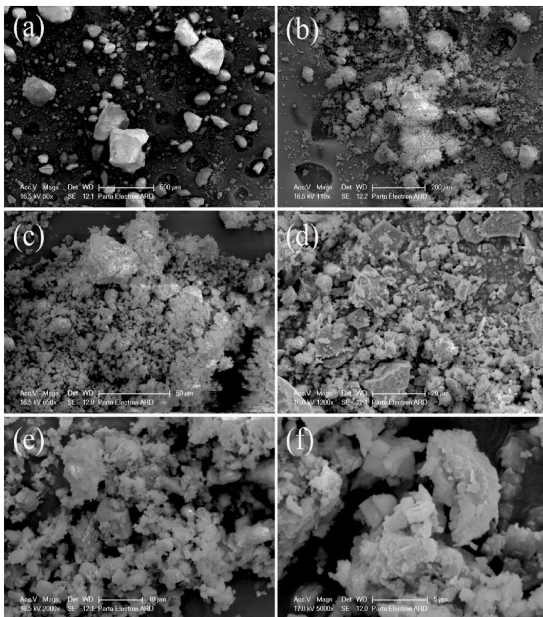
Fig. 3. SEM morphology of slag particles with different magnifications in different scales of (a) 500 \mu\text{m} , (b) 200 \mu\text{m} , (c) 50 \mu\text{m} , (d) 20 \mu\text{m} , (e) 10 \mu\text{m} , and (f) 5 \mu\text{m} .
