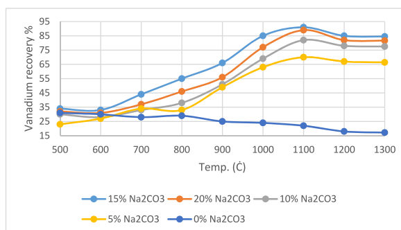
Fig. 6. Effect of roasting temperature and Na 2 CO 3 Wt. % on the V recovery.
