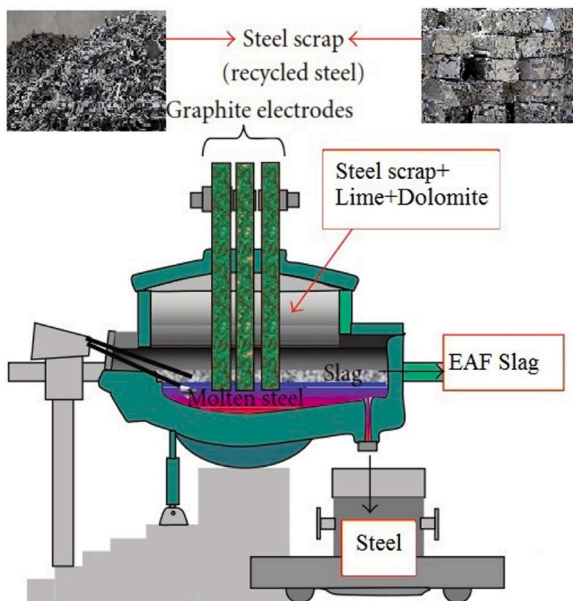
Fig. 1. The schematic drawing of EAF steelmaking process.
