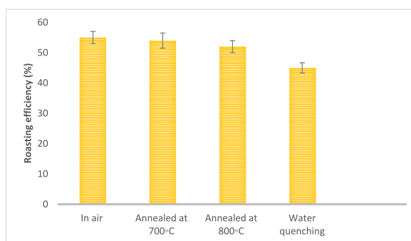
Fig. 9. Effect of cooling types on the roasting efficiency (%).
