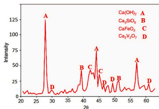
Fig. 4. XRD pattern of the slag sample.
