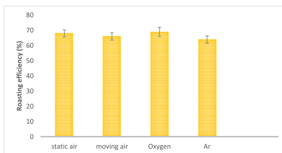
Fig. 8. Effect of roasting atmosphere on the roasting efficiency (%).
