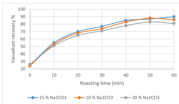
Fig. 7. Effect of sodium carbonate Wt. % and roasting time on the V recovery.
