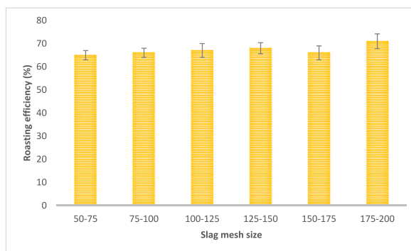
Fig. 5. Effect of slag mesh size on the roasting efficiency.
