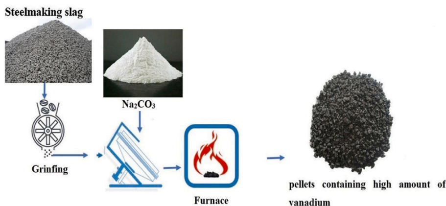
Fig. 2. Extraction process of V from the steel slag.
